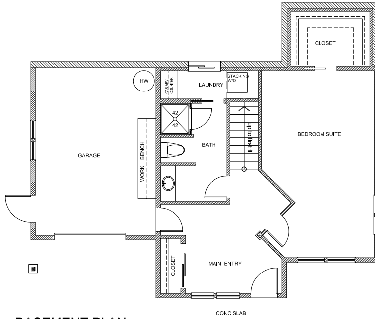
BASEMENT PLAN
