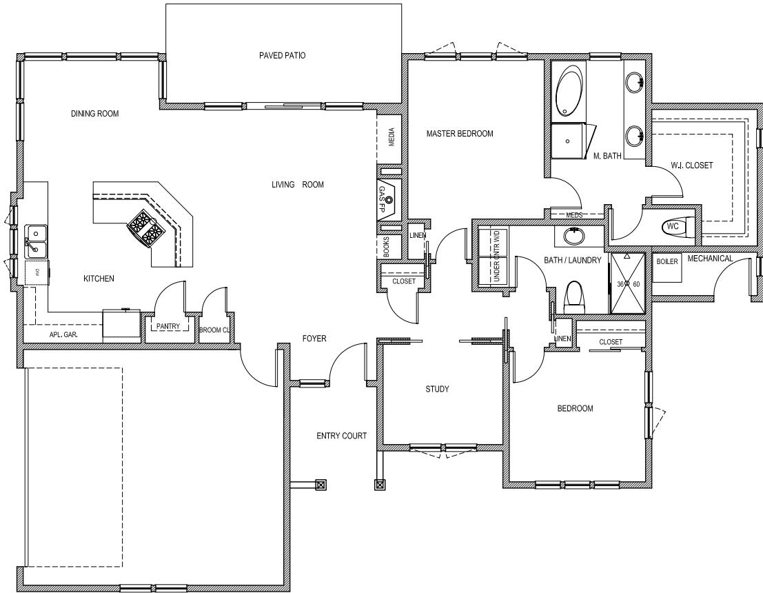
FLOOR PLAN
