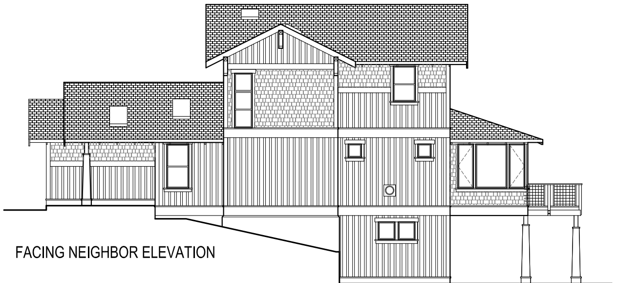
SIDE STREET / VIEW ELEVATION
