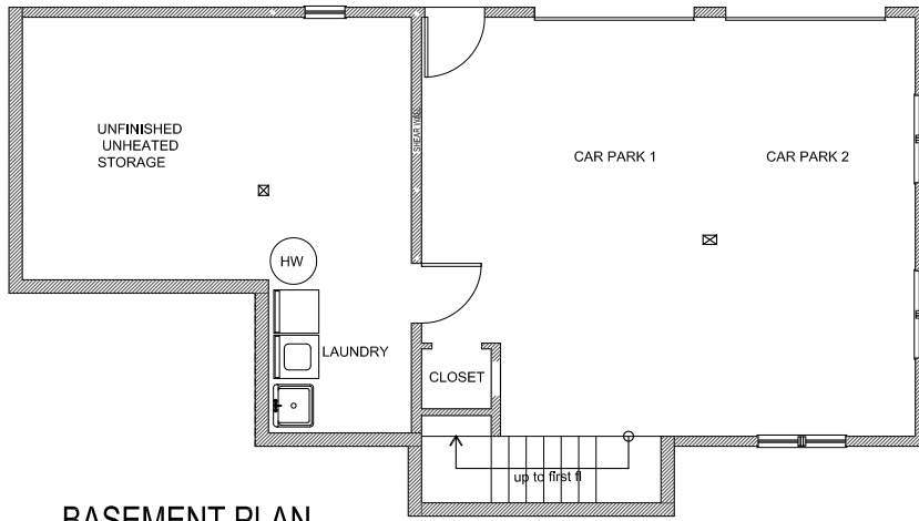
BASEMENT PLAN
