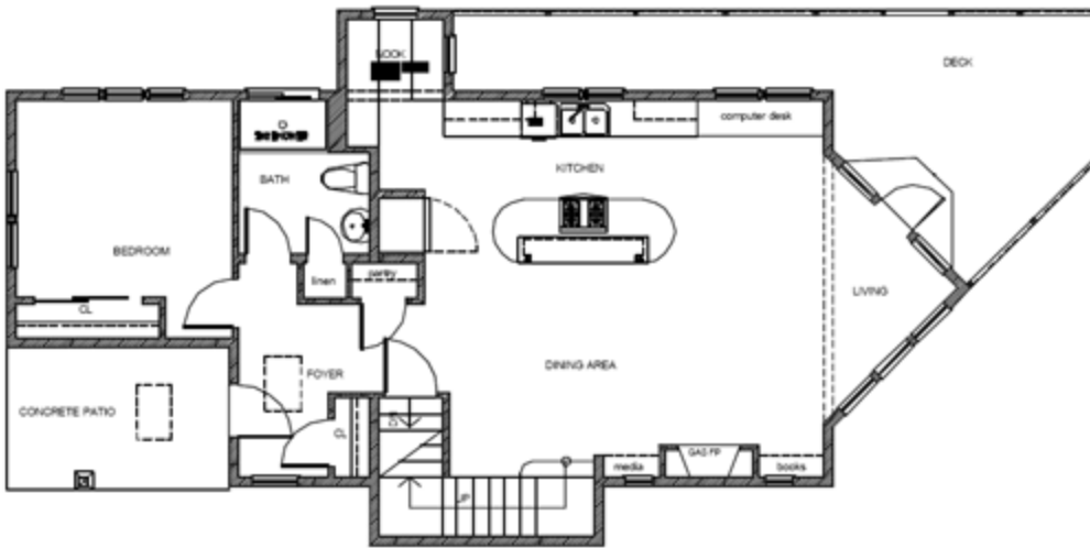
Main Floor
