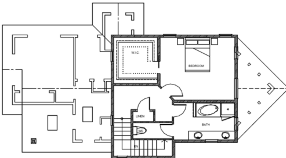
Upper Floor
