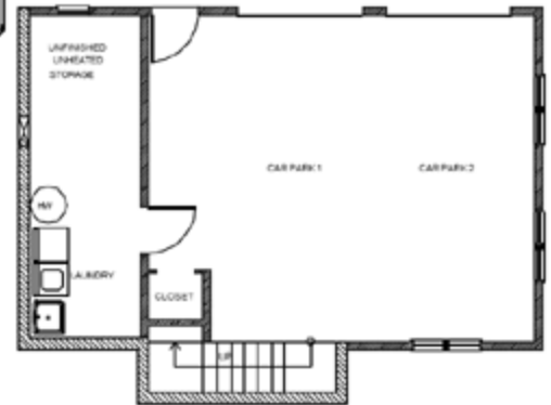
Basement Level
